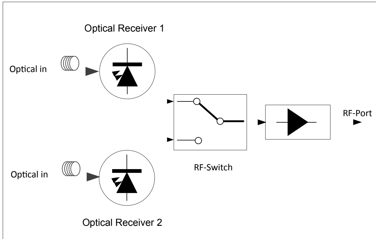
OFN200-FS Blockdiagram
