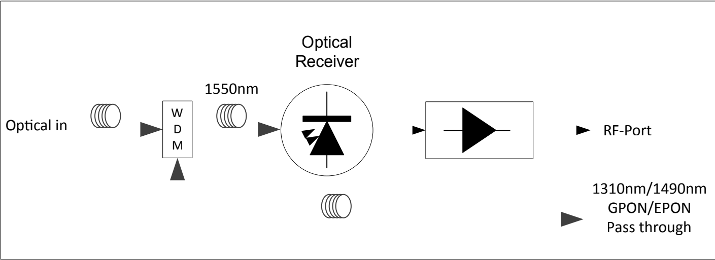
OFN100-FW Blockdiagram
