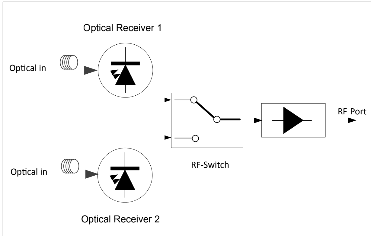
OFN100-FS Blockdiagram
