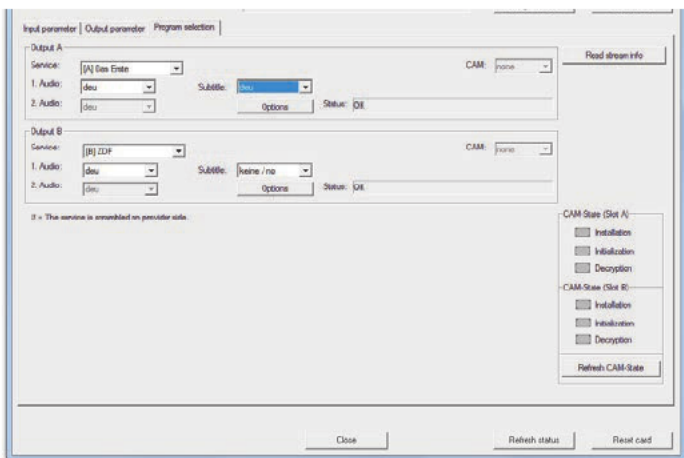
Figure 11: Selecting programmes
