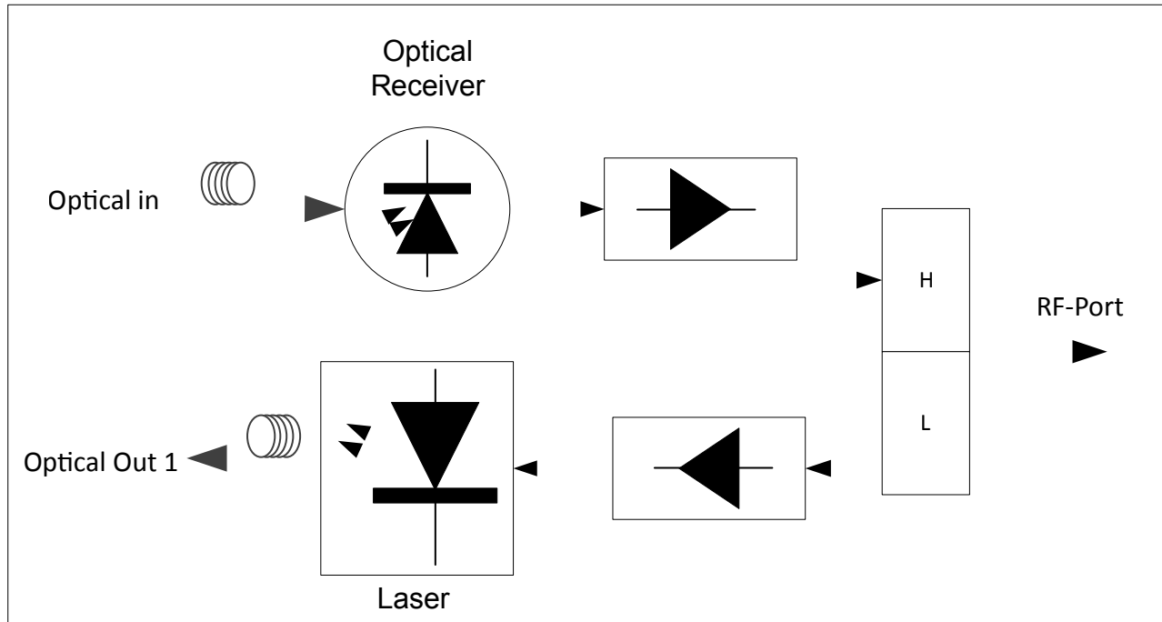
OFN200-FR Blockdiagram
