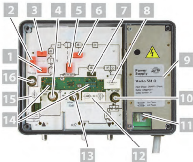
Fig. 2: VARIO 561 O amplifier, interior
