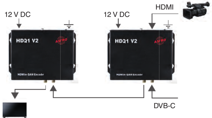
Fig. 4: Connection example with cascade connection
