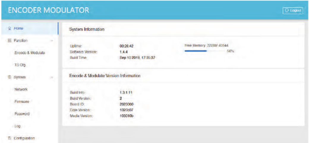
Fig. 6: Status overview
