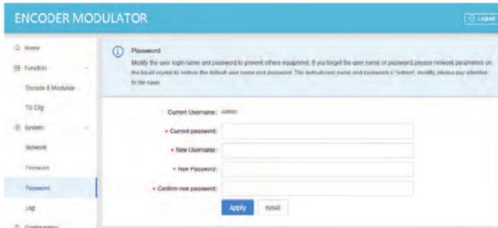
Fig. 12: Changing password
